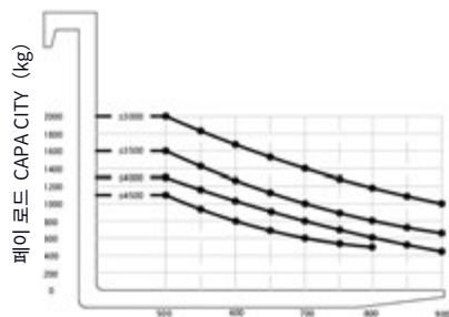
SE20-부하 곡선CAPACITY CHART (mm) 리프팅 높이LIFT HEIGHT (mm)
